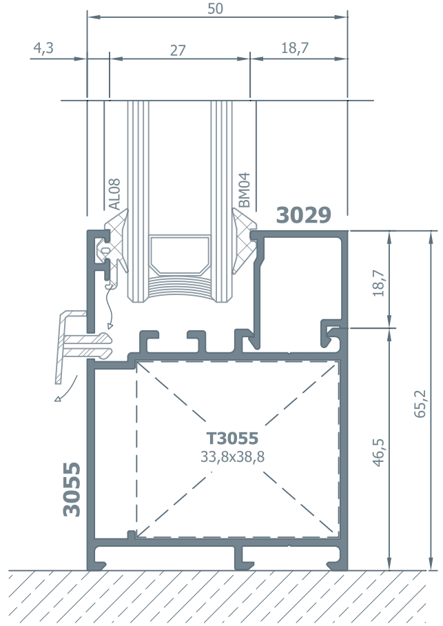
3.3 Detay Details
