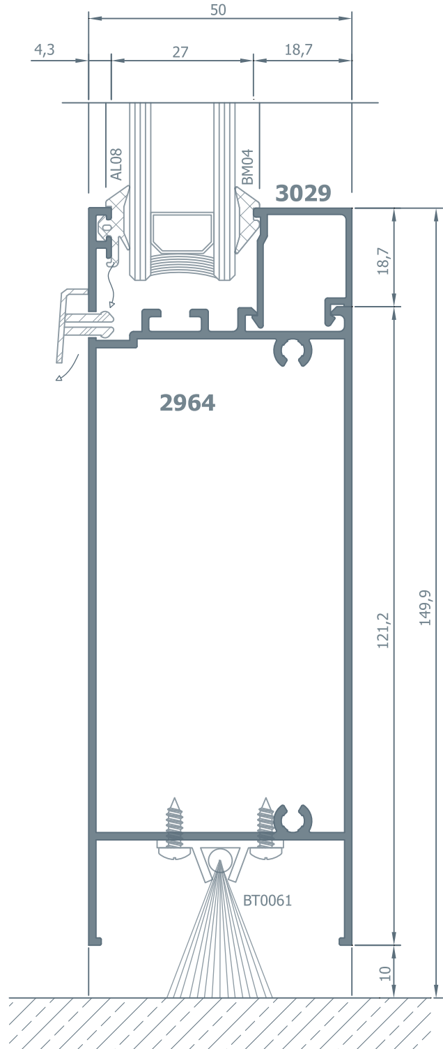
11.11 Detay Details
